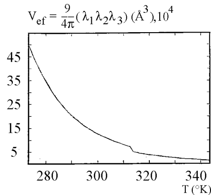
Fig. 2. Temperature dependence of the volume of lipid domains: V = \frac{9}{4\pi} \lambda_1 \lambda_2 \lambda_3 . The volume is determined by 3D superposition of the most probable de Broglie waves of lipid molecules or their fragments. Phase transition occurs in the region of 312K (39 o ) and accompanies by trance - gauche change of lipid conformation.
